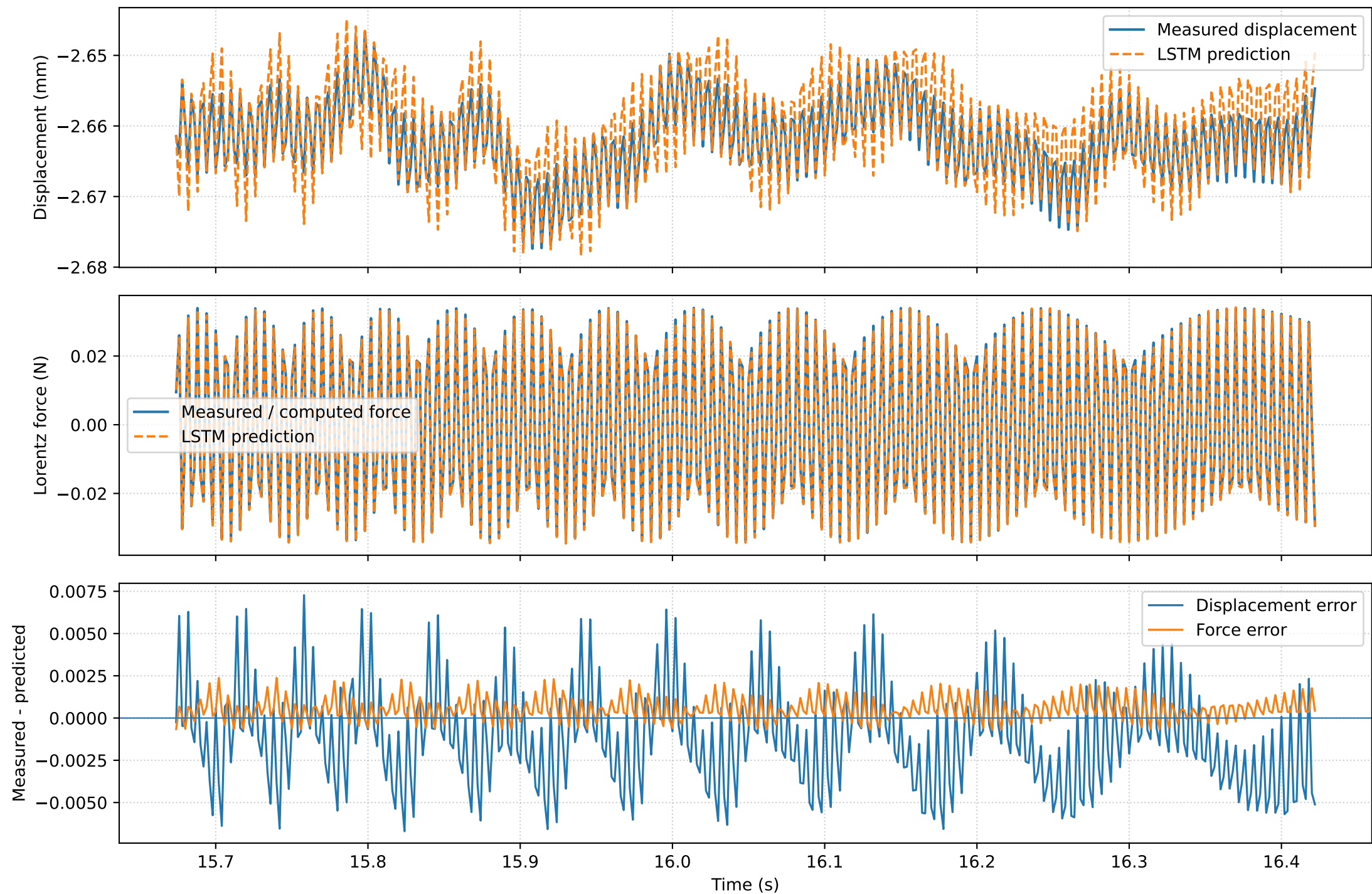
Zoomed LSTM tracking: Chirp_1 | center = 16.048 s | window = 0.750 s
